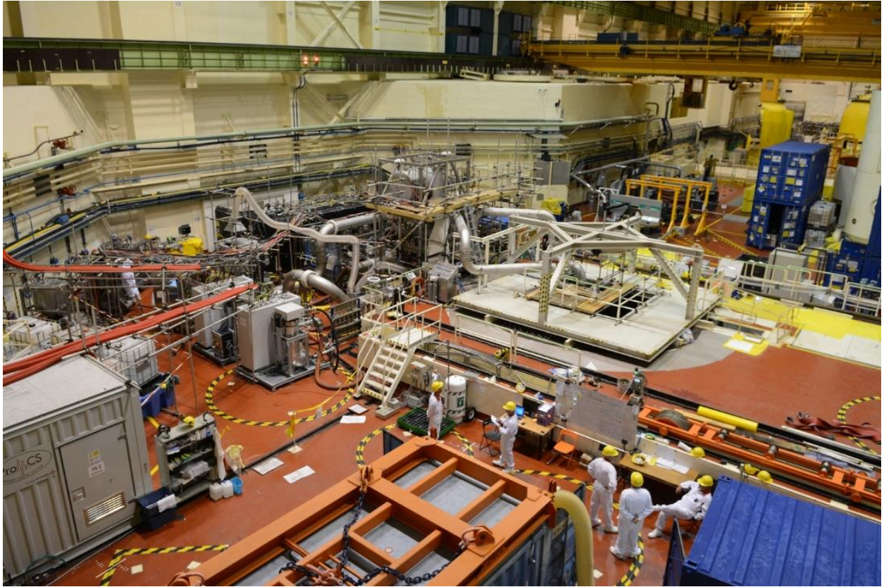
Figure 7: DFD line at Unit 2 V1 NPP.
